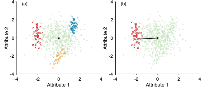
Fig. 2. Patterns found in the synthetic data (§II.§III). (a) Data with the embedded patterns highlighted. (b) Top ranked pattern. Light green circles are random data points, darker colored crosses the three embedded clusters.
