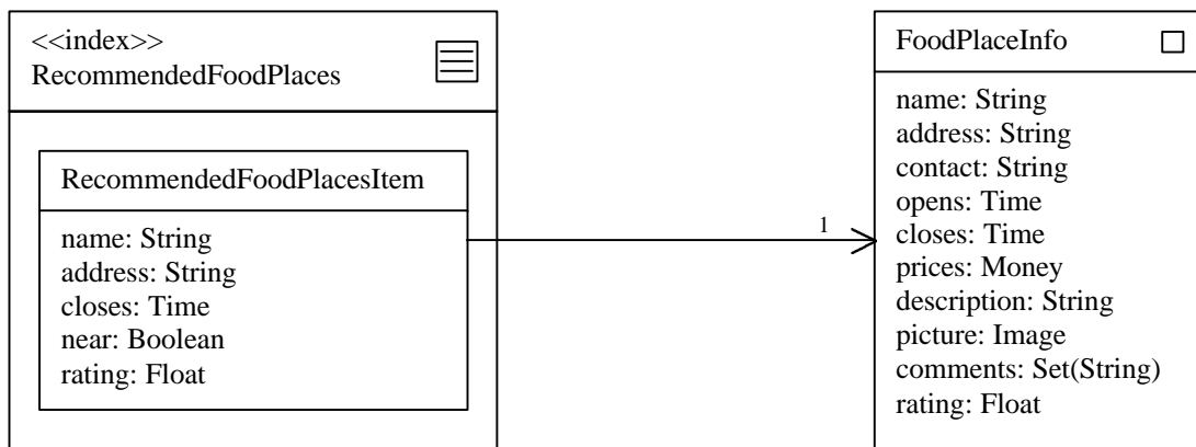
Figure 10. Adaptive Navigational Class Model.
