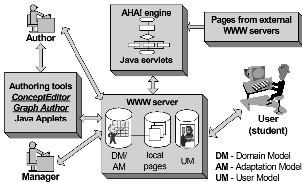
Figure 1. AHA! Architecture.
